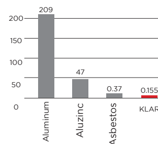
THERMAL CONDUCTIVITY
